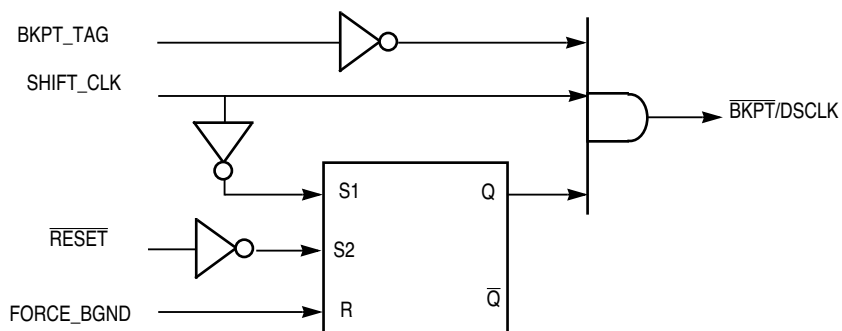
Figure 10-14 \overline{\text{BKPT}}/\text{DSCLK} Logic Diagram
