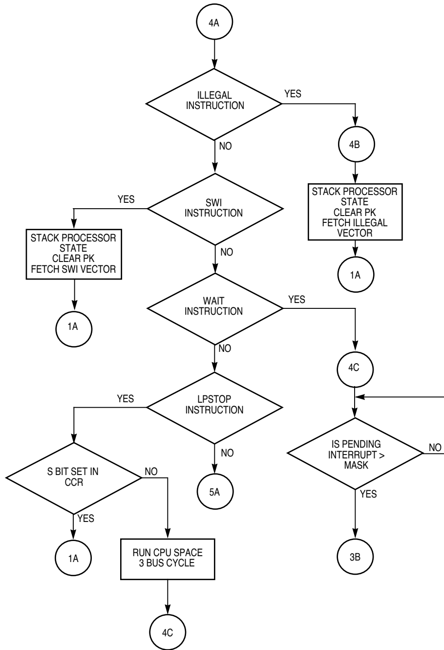
Figure 9-2 (Sheet 4 of 5) Exception Processing Flow Diagram
