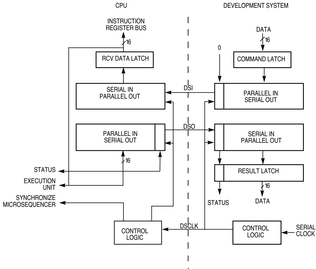
Figure 10-9 BDM Serial I/O Block Diagram
