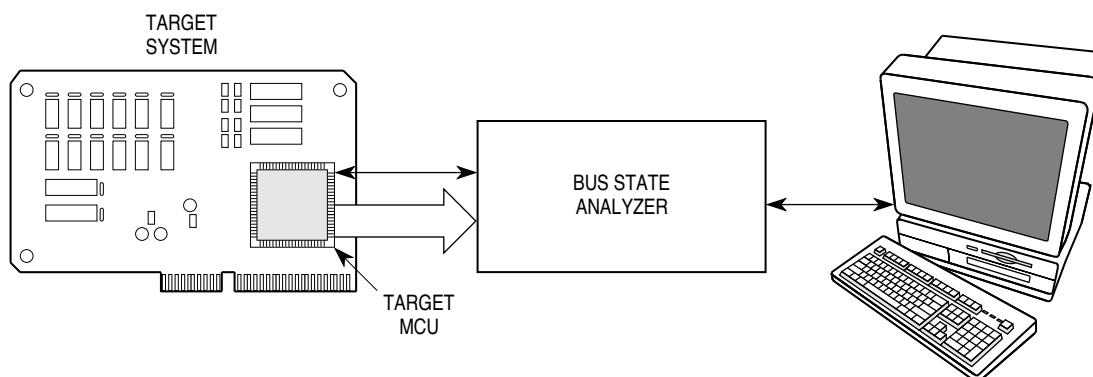
Figure 10-5 Bus State Analyzer Configuration
