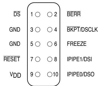
Figure 10-16 BDM Connector Pinout
