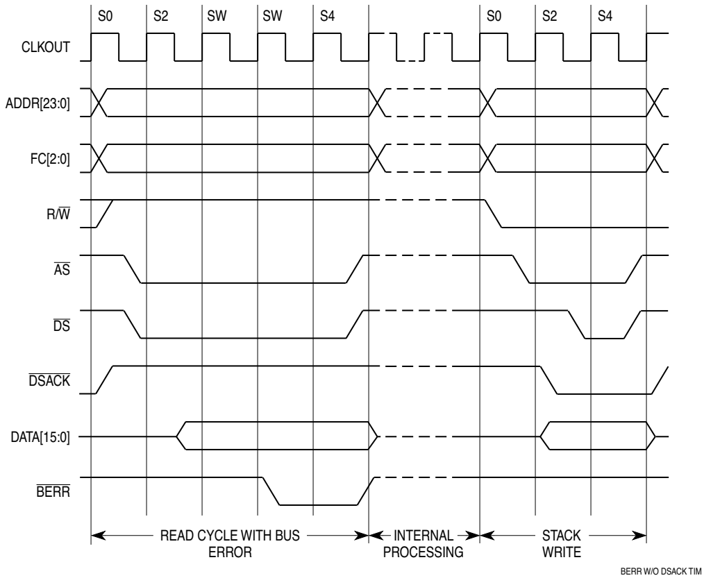
Figure 5-31 Bus Error Without DSACK
