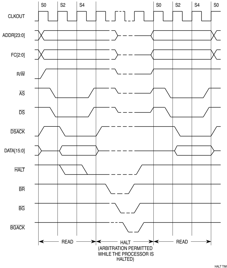
Figure 5-35 \overline{\text{HALT}} Timing
