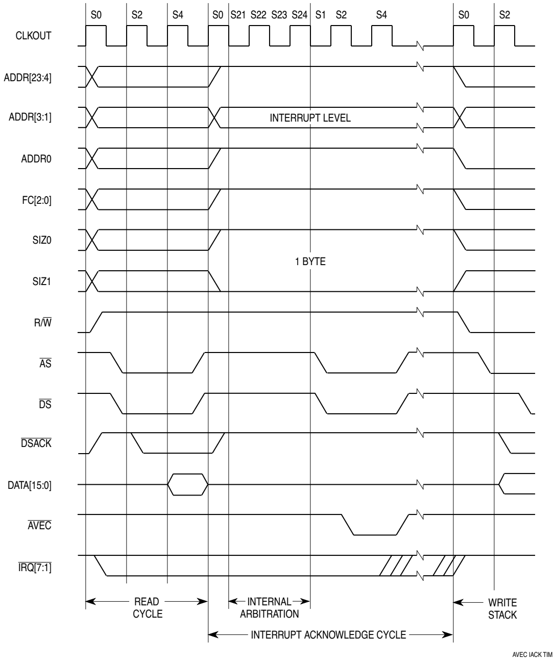
Figure 6-5 Autovector Timing
