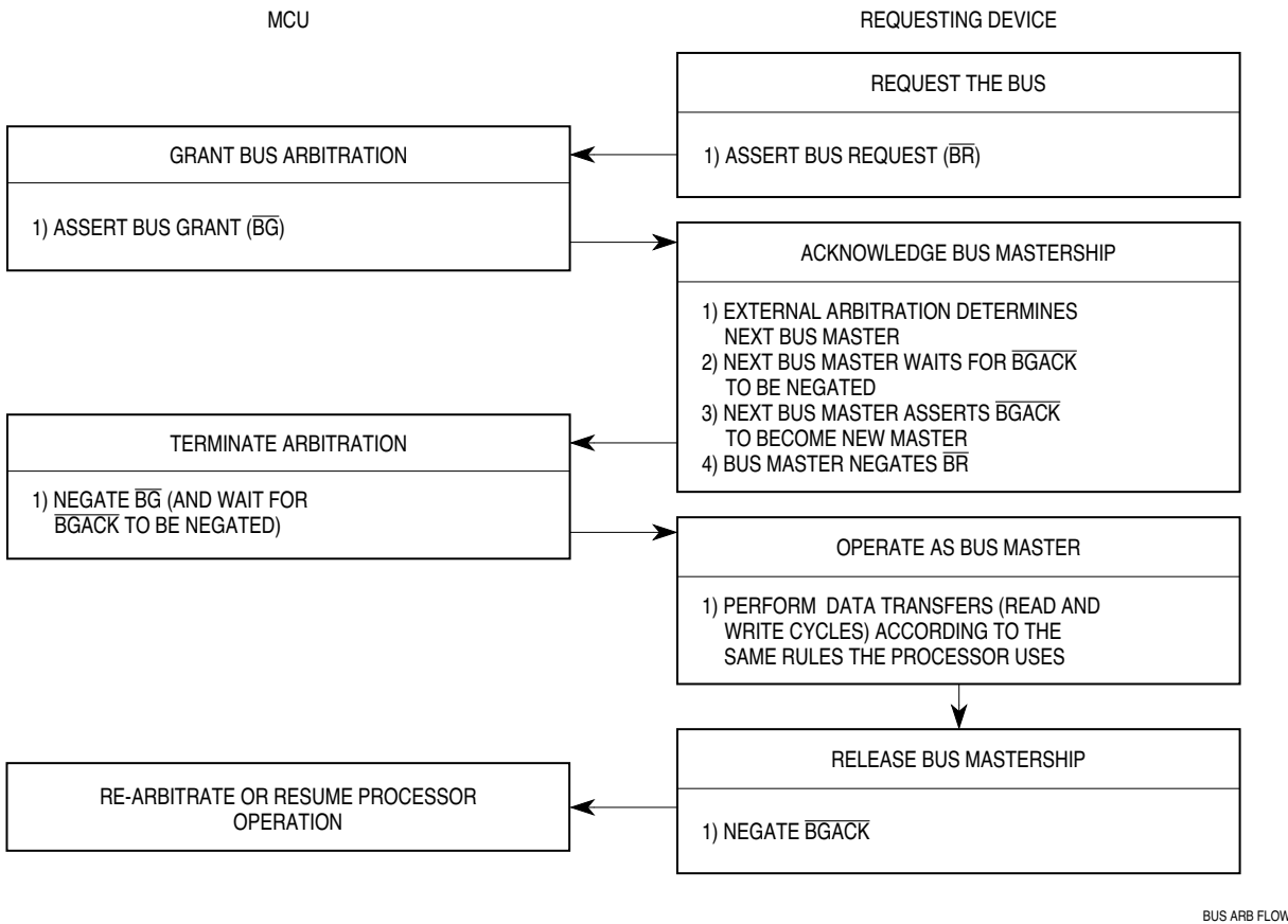
Figure 5-36 Bus Arbitration Flowchart for Single Request
