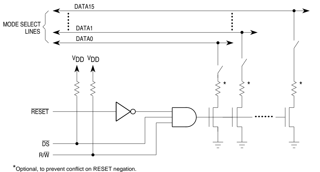
DATA BUS MODE DECODE
