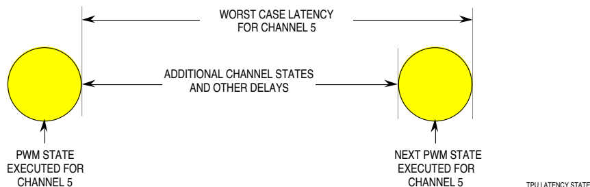
Figure C-1 Worst-Case Latency for PWM
