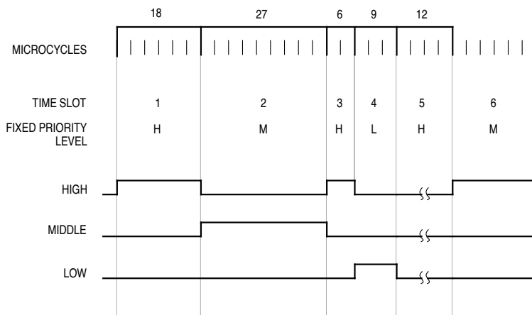
Figure 3-3 Time-Slot Variation
